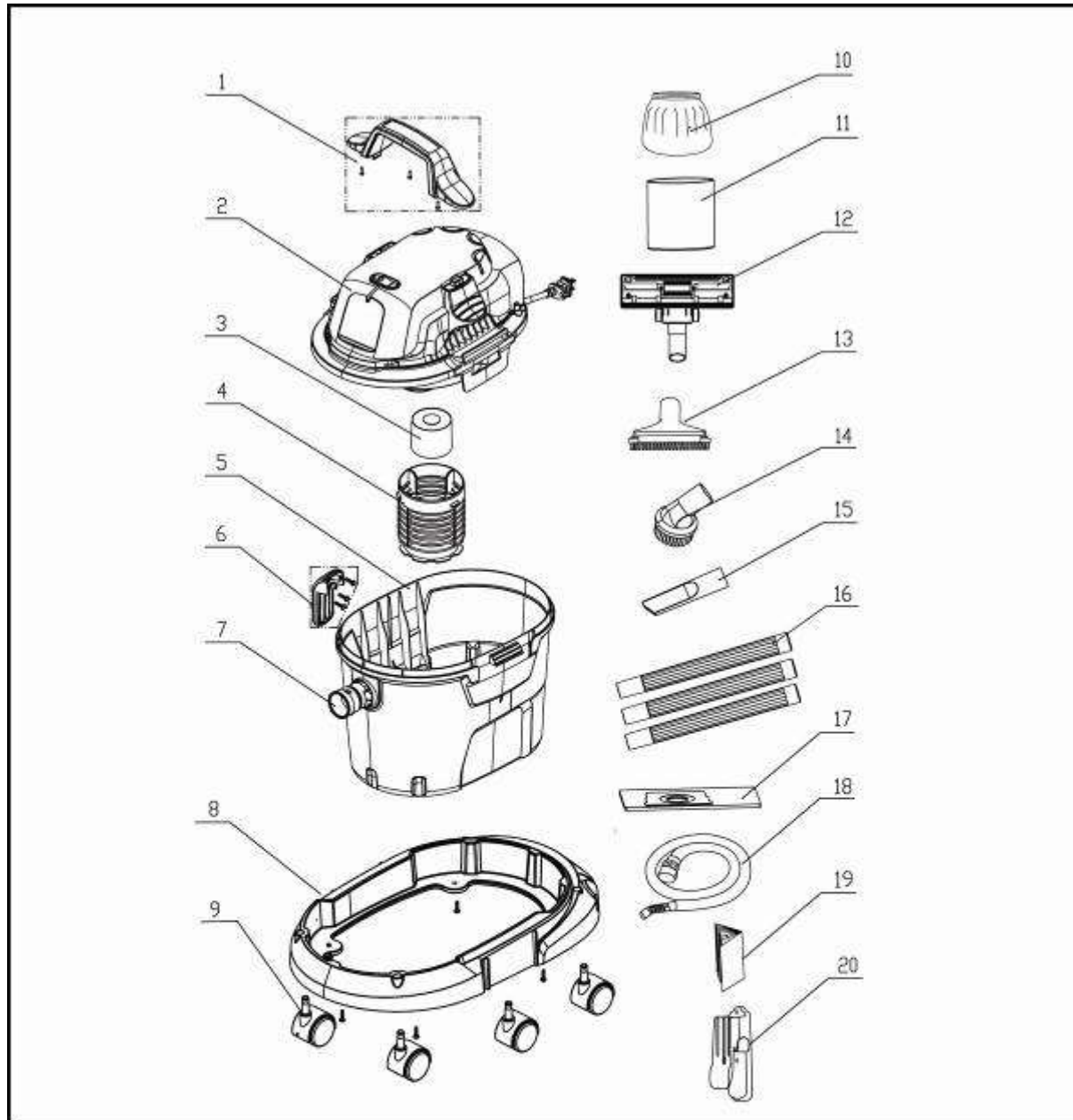
VHB305M Parts List
